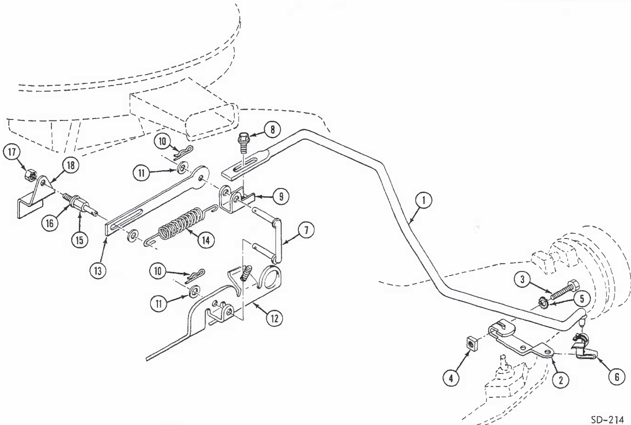
Figure 11-6 Transmission-Throttle Valve Linkage
