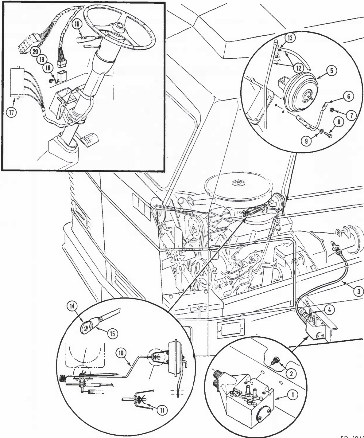
Figure 11-5. Cruise Control Installation.
