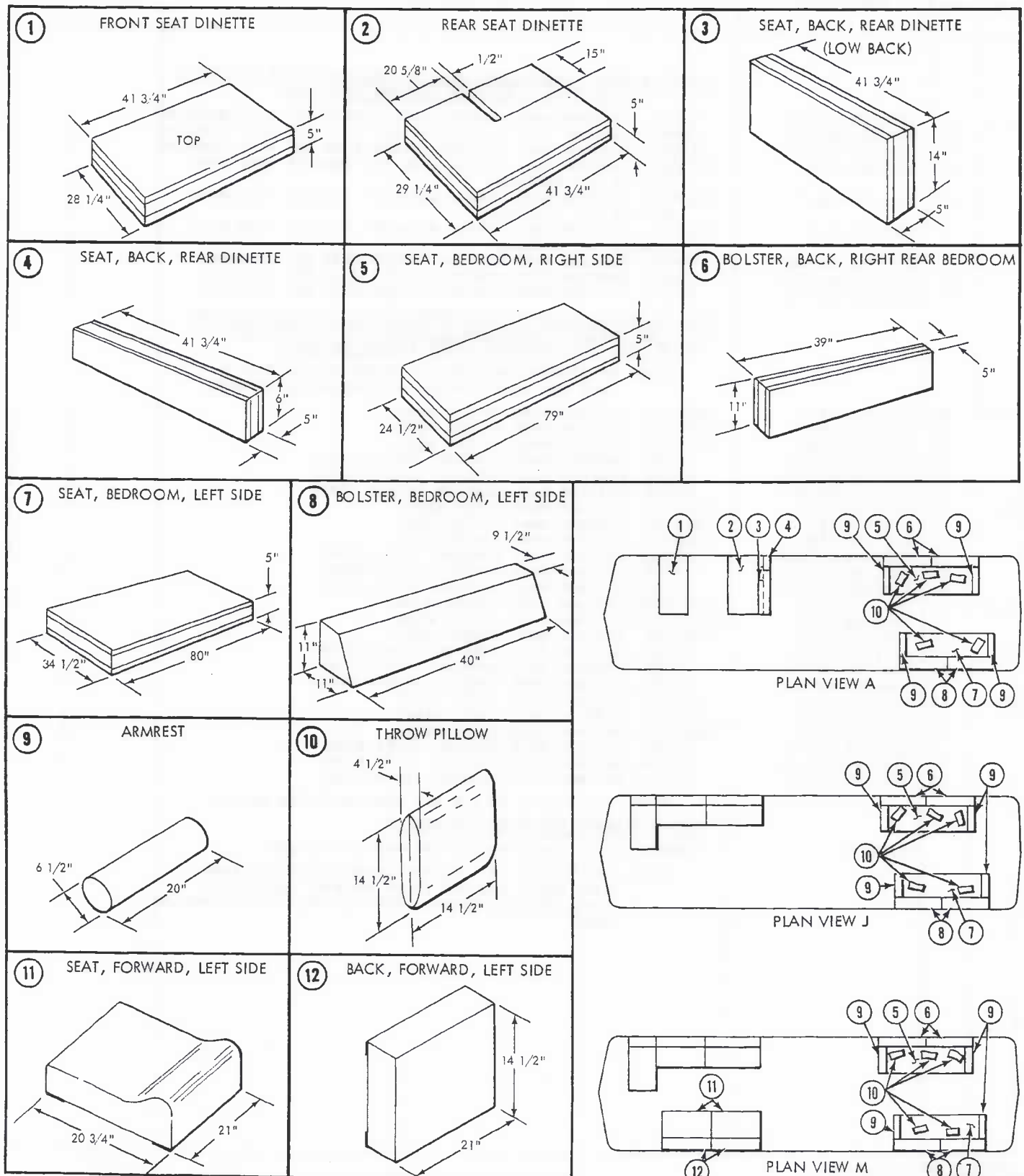
Figure 32-1.1. Cushions and Bolsters (Coach 00874 and Up)
