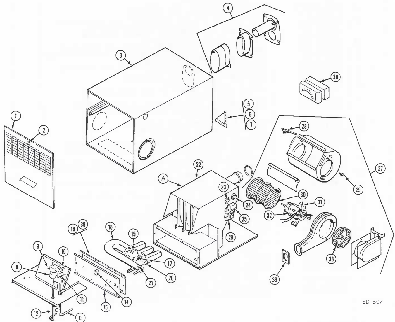
Figure 36-2. Coleman Furnace Assembly (Coach 00001 to 00829)
